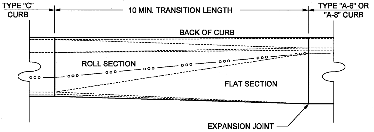
PLAN VIEW
