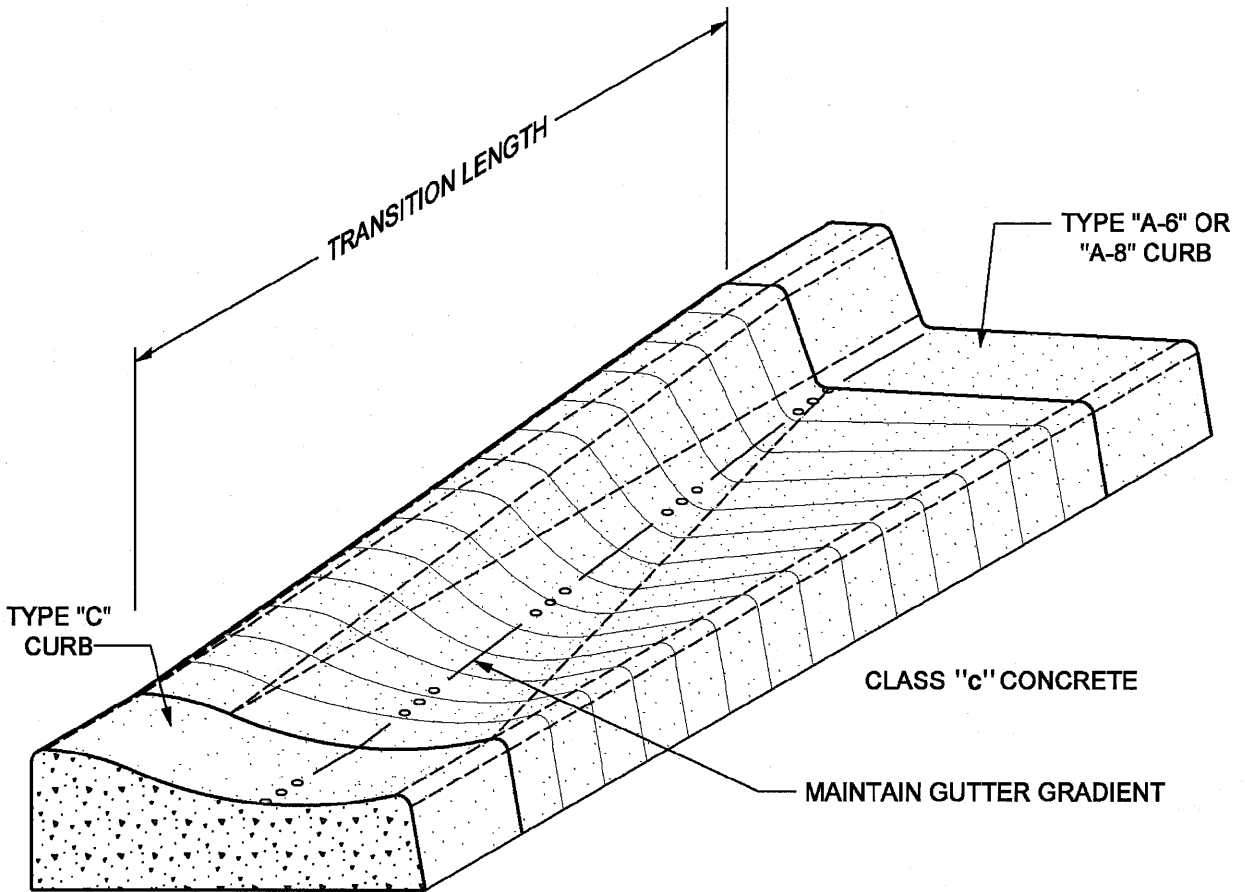
ISOMETRIC VIEW
