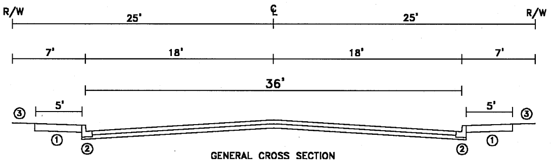
GENERAL CROSS SECTION
