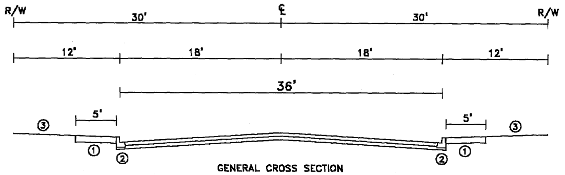
GENERAL CROSS SECTION
