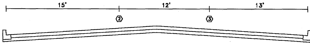
LANE WIDTHS AT INTERSECTION 6
