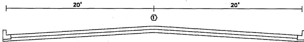
MID-BLOCK LANE WIDTHS
