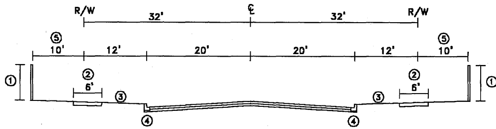
GENERAL CROSS SECTION
